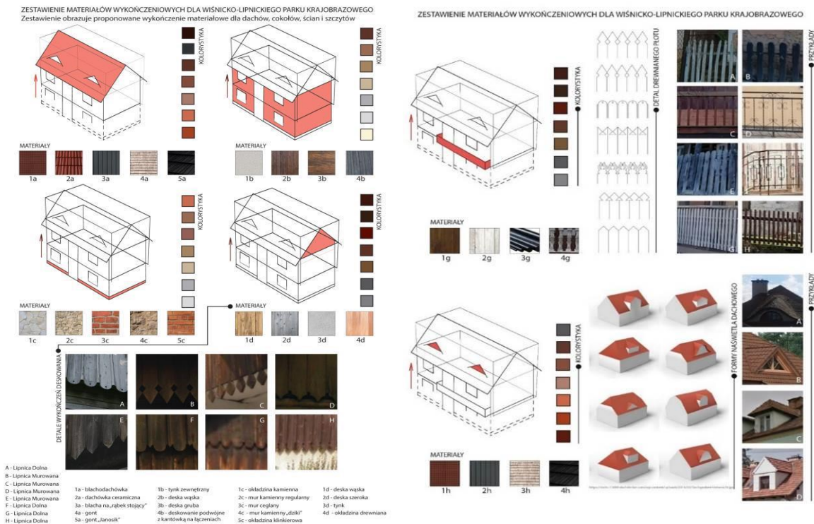
Fig. 7. A list of building elements with guidelines based on preserved characteristic elements. Source: Śródulka -Wielgus J. et al. 2020, pp. 159-160, by authors,
